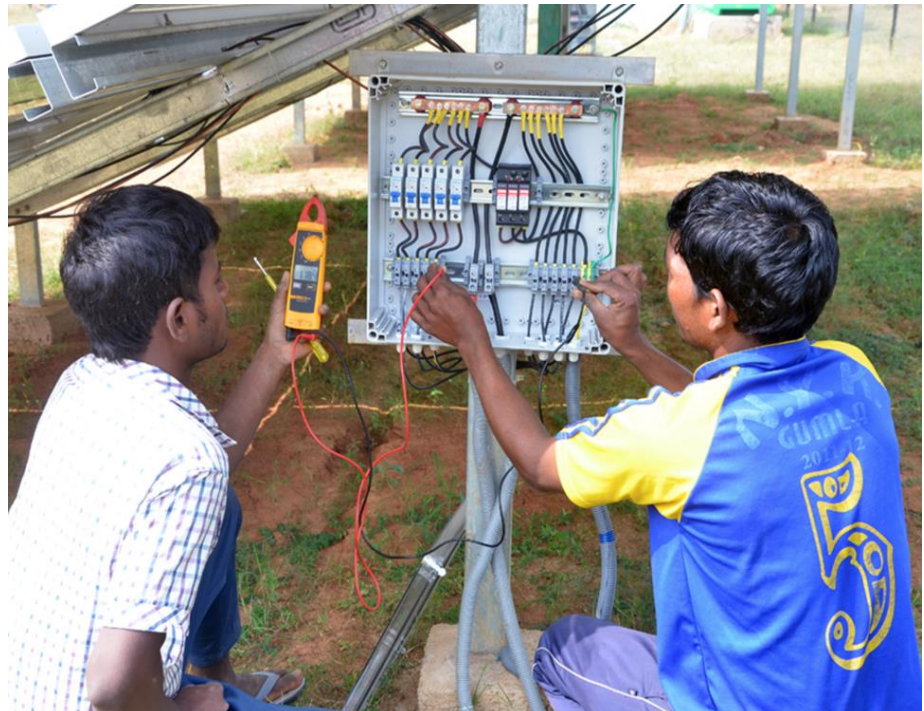
Mini-grid operator and engineer test the mini-grid power supply Source: Mlinda, 2019
